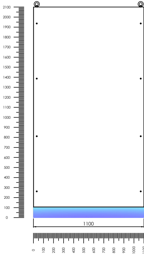
Back View
